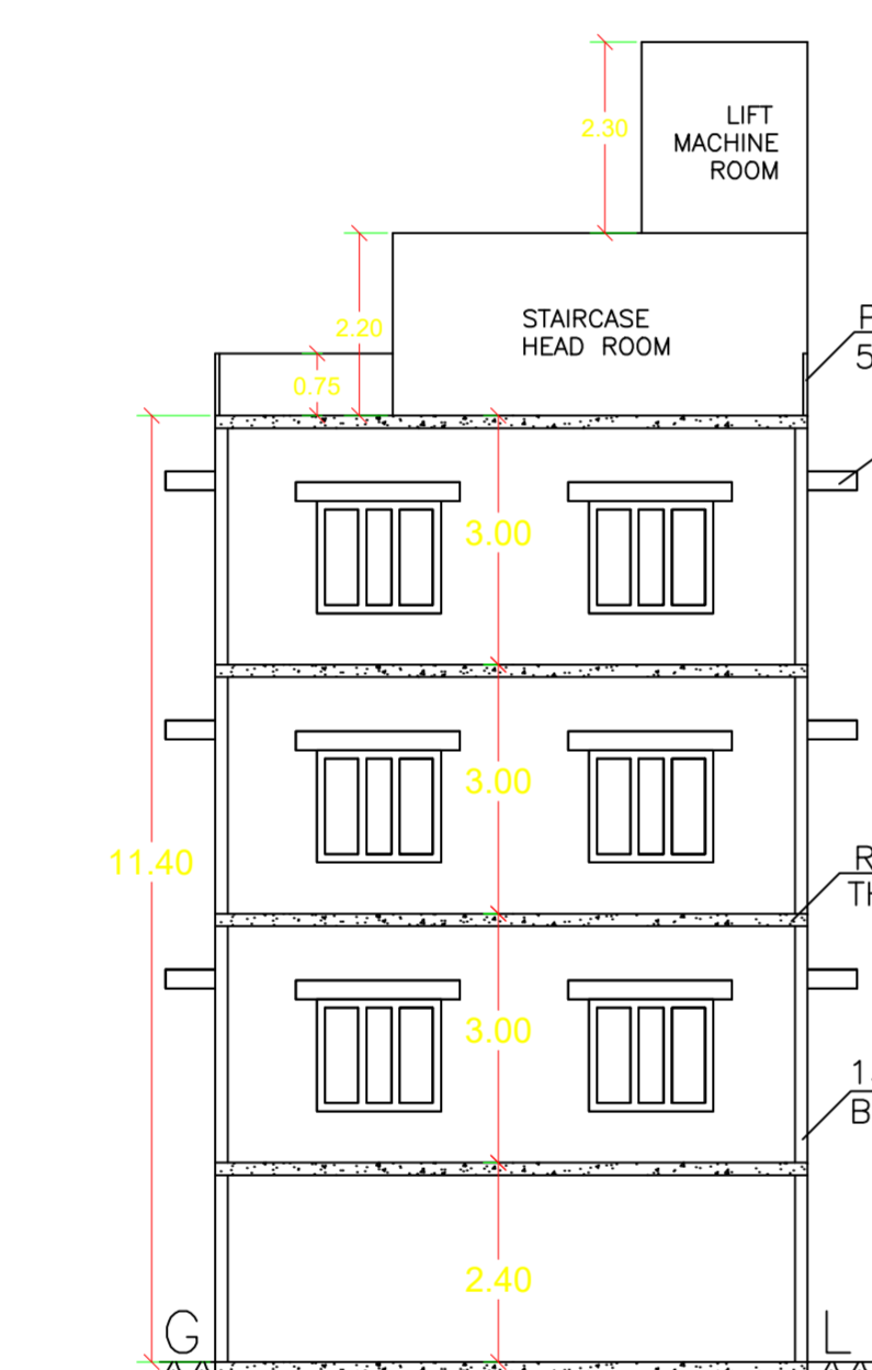
SECTIONAL ELEVATION AT X-X
