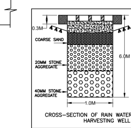
CROSS-SECTION OF RAIN WATER HARVESTING WELL
